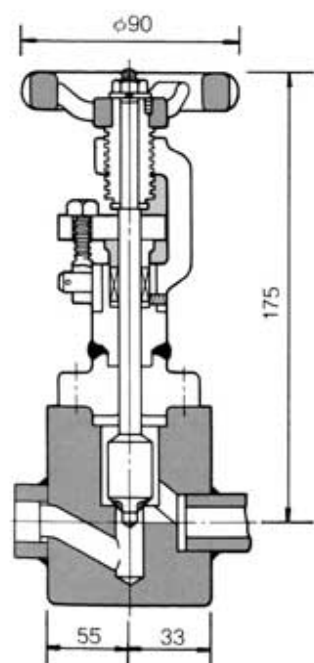
NKG Drain Valve DV15
