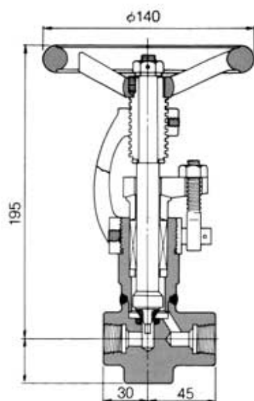
NKG Drain Valve DV18
