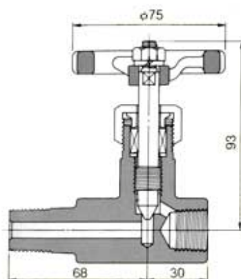
NKG Drain Valve DV21
