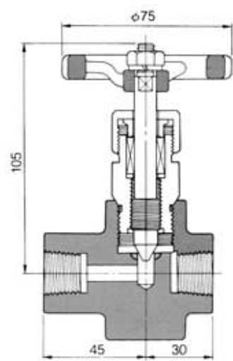
NKG Drain Valve DV24
