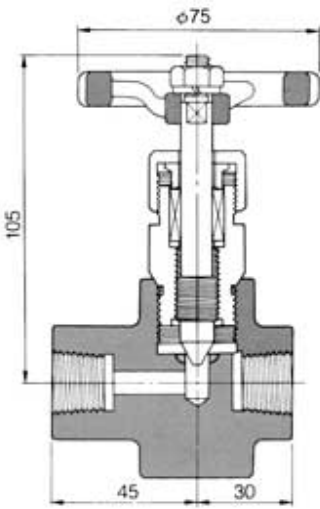
NKG Drain Valve DV25
