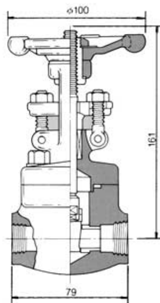
NKG Drain Valve DV51
