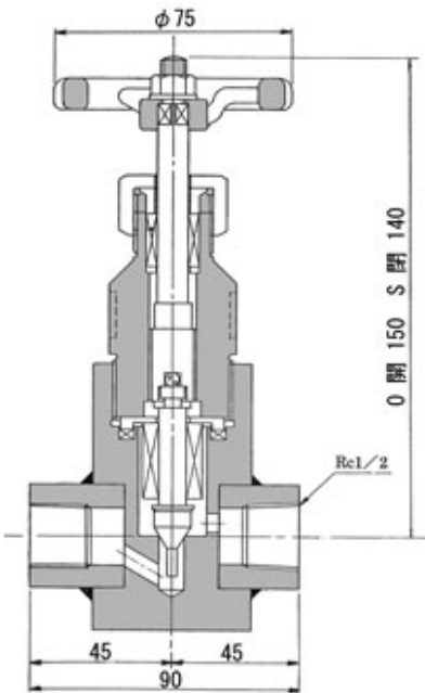
NKG Drain Valve DV61
