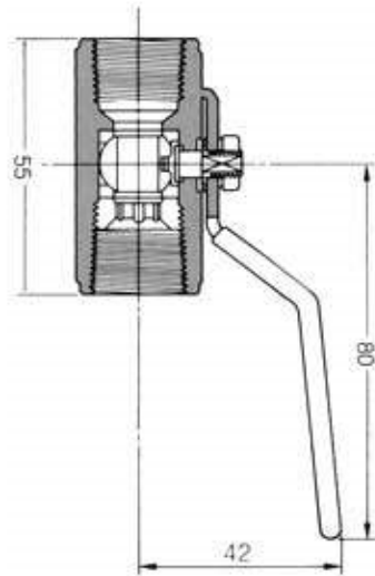
NKG Drain Valve DV70
